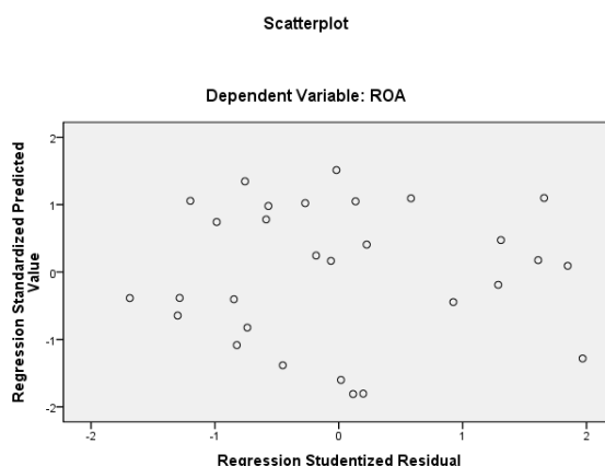
Gambar 1. Scatterplot Hasil Penelitian
